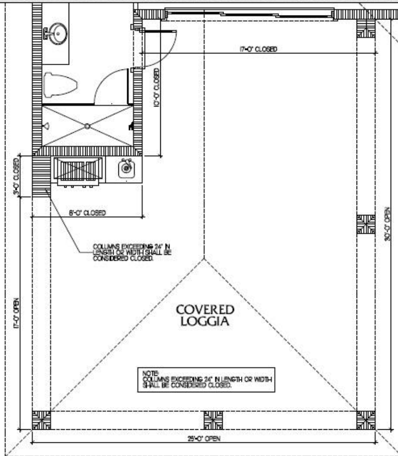
FIGURE 1 COVERED LOGGIA(PARTIAL CREDIT CALCULATION EXAMPLE)
